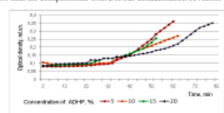
Fig. 2. Changes in the optical density of compositions with the addition of ADHP over time.
